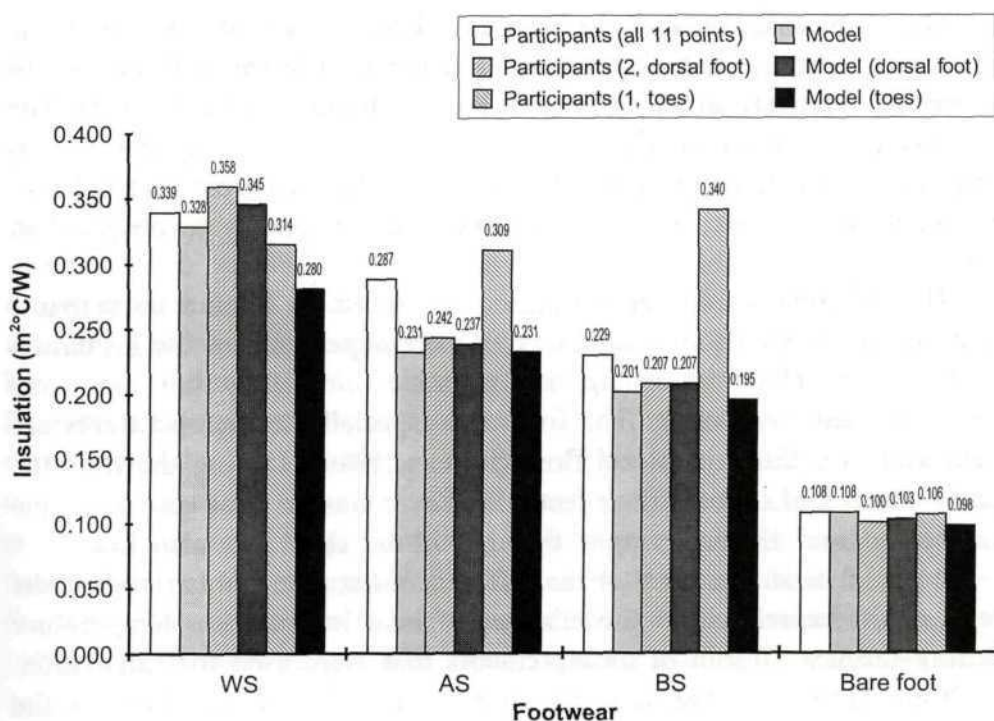
Figure 2. Insulation values from measurements on participants and on the thermal foot model. The insulation values on participants are based on all (11) points, 2 points (5 and 6) on the dorsal foot, and 1 point (1) on the big toe. Notes. WS—warm footwear for winter use, AS—a leather boot without lining, BS—a rubber boot without lining.
